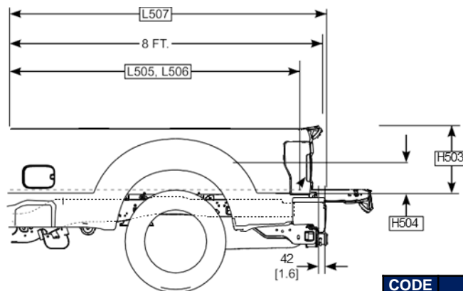
8 FT. BOX
