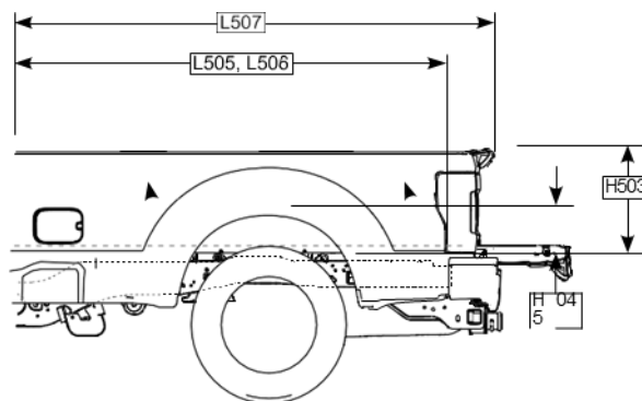
6.75 FT. BOX
