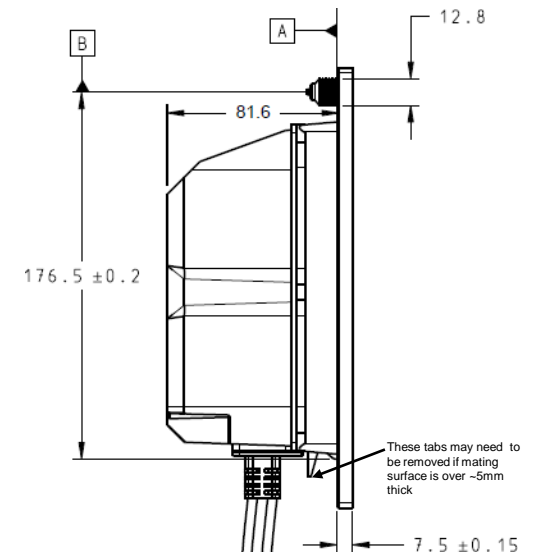
AUX OUTLET MATING SURFACE
