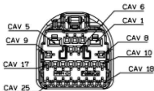
MATING FACE VIEW
