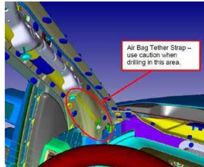
Figure 3: Air Bag Tether
