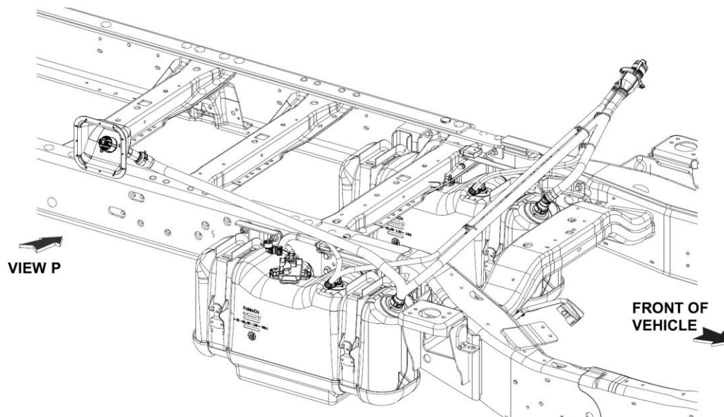
PICKUP BOX DELETE / REMOVAL (WIDE FRAME) TYPICAL INSTALLATION
