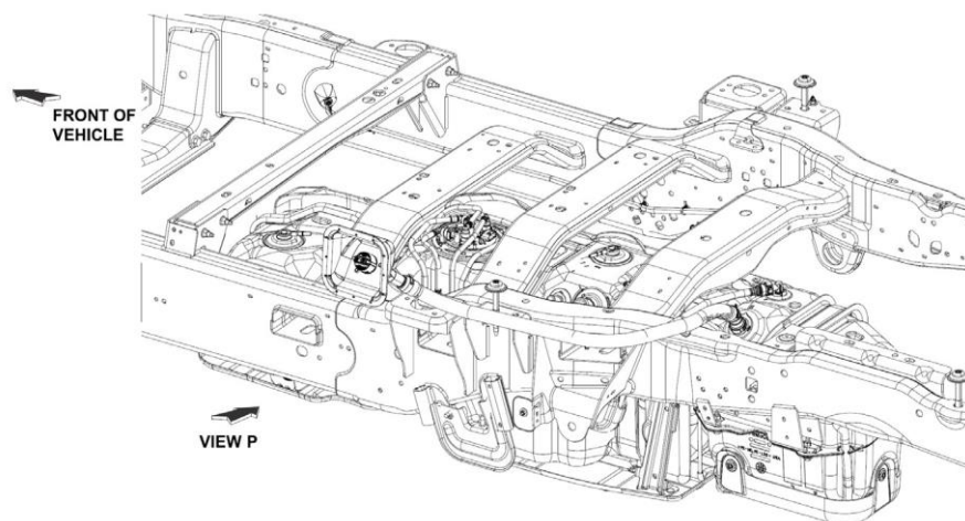
PICKUP BOX DELETE / REMOVAL (WIDE FRAME) TYPICAL INSTALLATION
