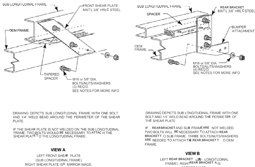
FIGURE A - TECHNIQUE #1 SHEAR PLATES W/LONGITUDINAL SUB STRUCTURE
