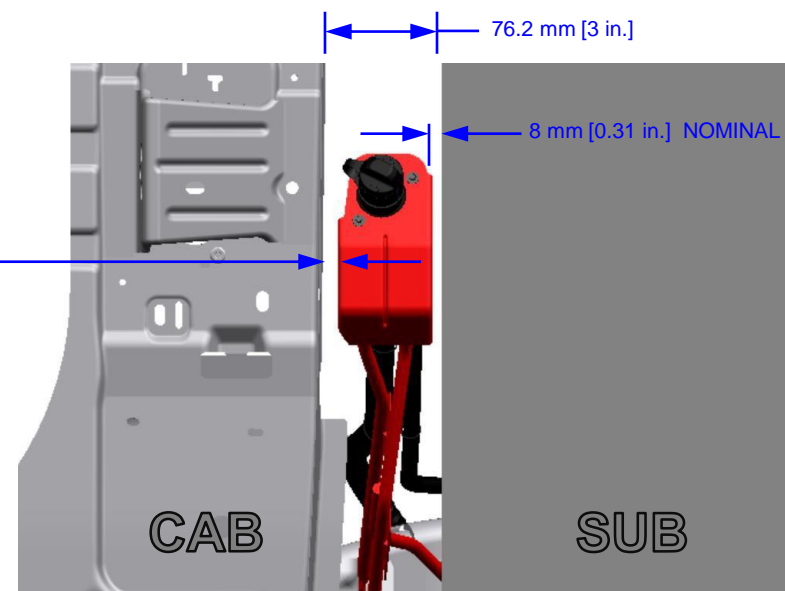
SIDE VIEW
