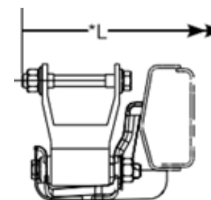
SECTION A ENLARGED
