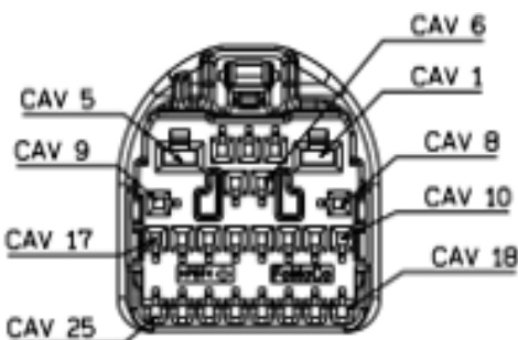
MATING FACE VIEW
