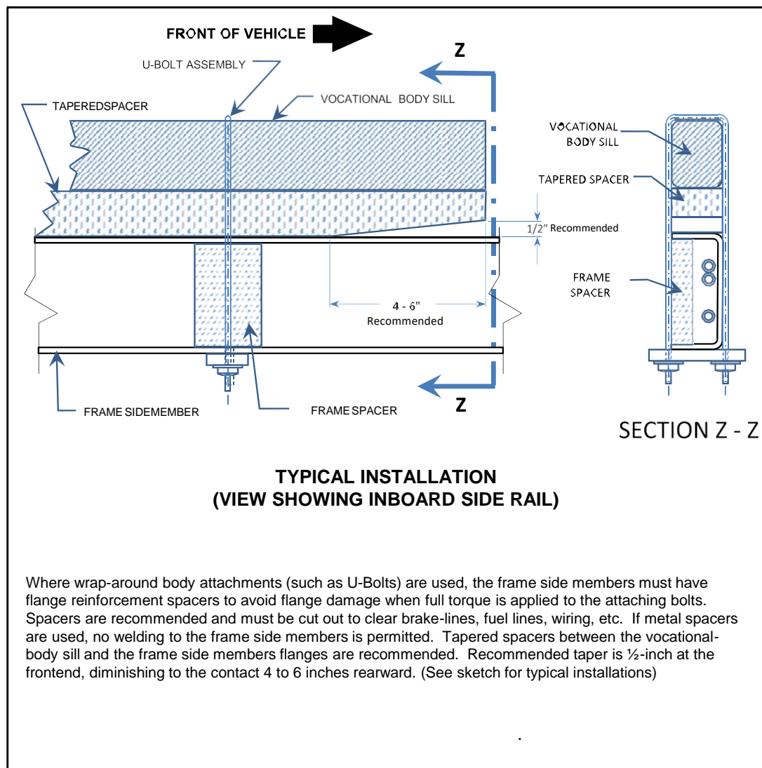
FIGURE C - CHASSIS CAB SUB-MOUNTING SPACER
