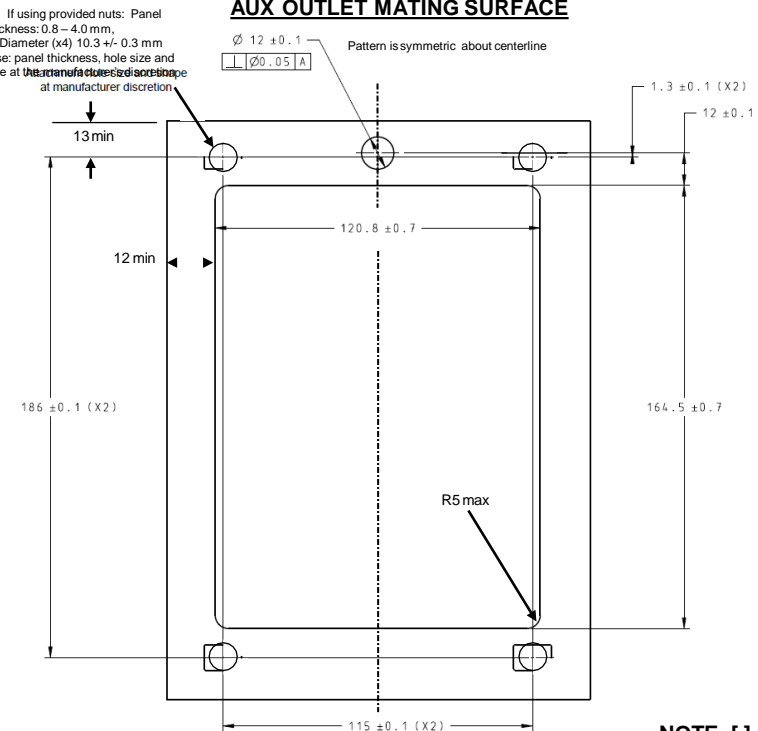
AUX OUTLET MATING SURFACE
