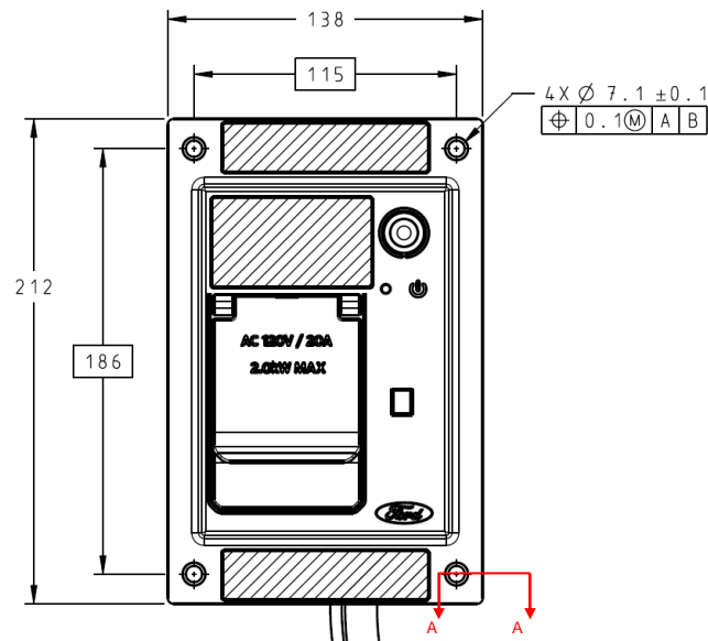
AUX OUTLET MATING SURFACE
