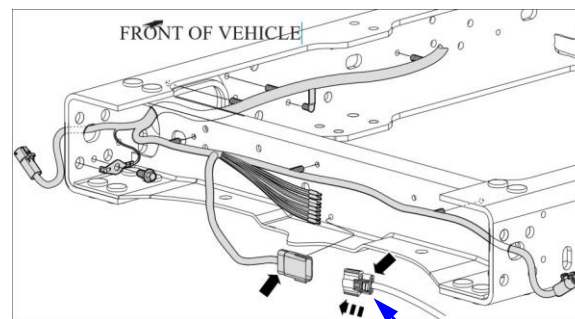
ITEM F - WIRE HARNESS
