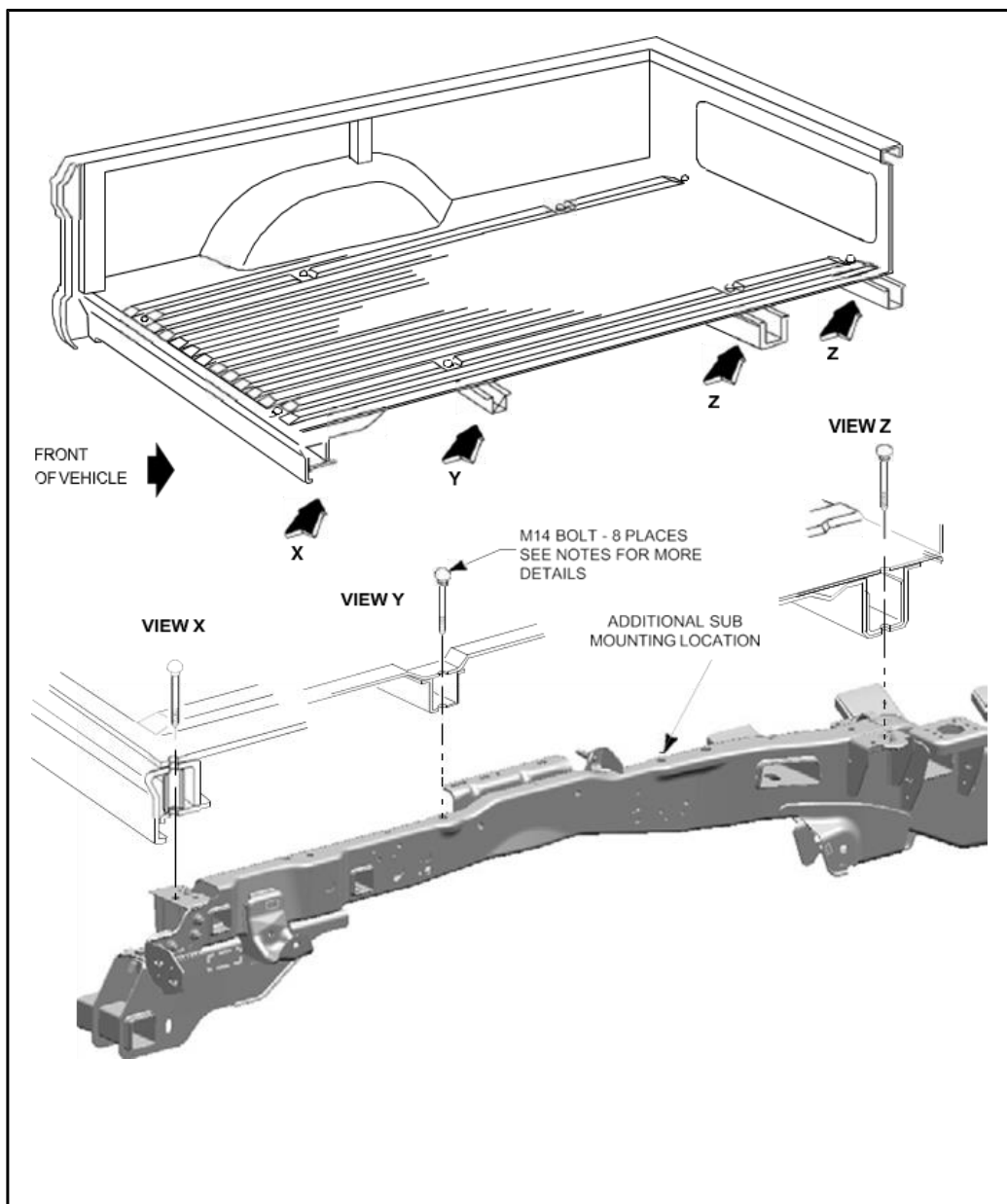
FIGURED – TOP-BOLTING SUB-Mounting for Pickup Box Removal
