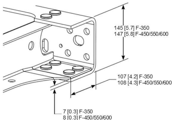
END OF FRAME
