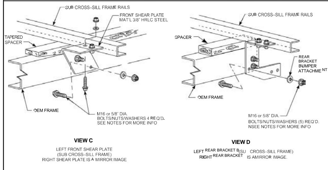
FIGURE B - TECHNIQUE #2 SHEAR PLATES W/LATERAL SUB STRUCTURE
