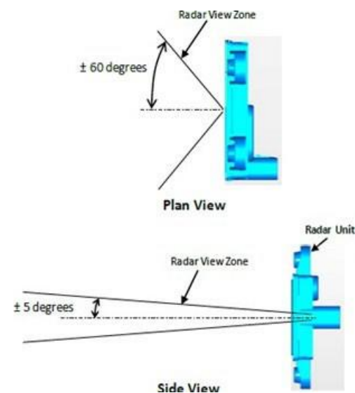
RADAR - FIELD OF VIEW' (CAD File: FNA6220214)
