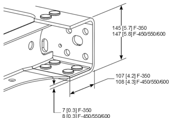
END OF FRAME
